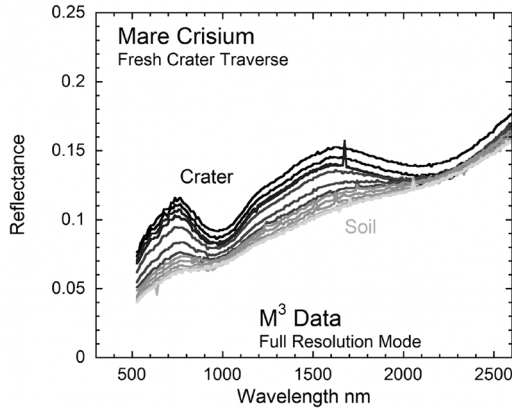
Figure 2. Moon Mineralogy Mapper ( M^3 ) data of a traverse across a fresh crater in Mare Crisium. Sampling radially across a fresh impact crater demonstrates the systematic effect of space weathering: the background soil is lower in reflectance and redder (steeper spectral slope) with reduced absorption bands compared to the fresh material exposed by the impact (modified from Noble and Pieters 2016).
