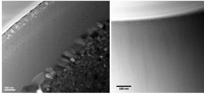
Figure 5. TEM images of npFe in olivine and pyroxene craters shown in Figures 4b,c. NpFe (black specks) is abundant throughout the olivine glass on the left, but only at the uppermost surface in the pyroxene sample on the right.
