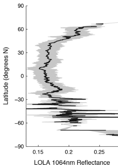
Figure 13. Average LOLA 1064 nm reflectance for the lunar maria vs. latitude. The reflectance is lowest near the equator and generally higher with increasing latitude (where the solar wind flux is lower), a pattern that holds when the maria are further subdivided by composition. After Hemingway et al. (2015).
