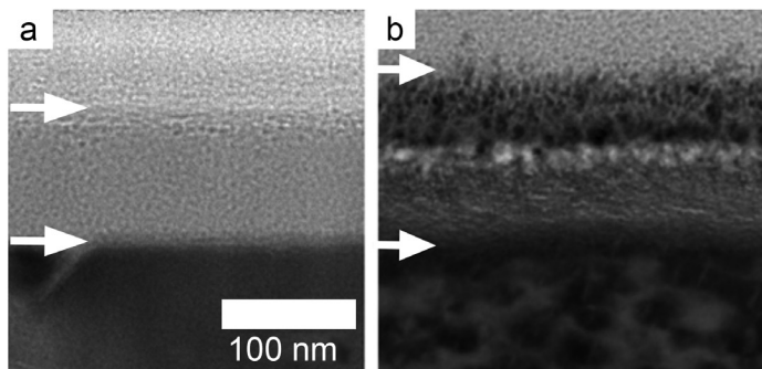
Figure 19. Transmission electron microscope images of the upper 400 nm of plagioclase (a) and ilmenite (b) single crystals prepared by focused ion beam (FIB) cross sectioning after they were ion irradiated in the laboratory with 4 keV He + ions and coated with amorphous carbon. (a) A conventional bright-field TEM image of an An 90 lunar plagioclase prepared from an interior thin section of lunar basalt 70035 and ion irradiated to a final He + fluence of 1.2 \times 10^{17} ions/cm 2 , (b) a bright-field STEM image of a synthetic ilmenite (FeTiO 3 ) grain ion irradiated to a final He + fluence of 3 \times 10^{17} ions/cm 2 . Arrows show the upper and lower boundary of the ion damaged layer in each sample, which in plagioclase is uniformly amorphous with a thin implantation bubble layer at the top. The ilmenite shows three distinct nano-crystalline/partially ion damaged layers, including an uppermost layer containing abundant nanophase Fe 0 .
