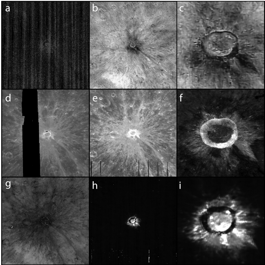
Figure 11. New views of fresh crater Giordano Bruno highlight the effects of space weathering across the spectrum. 10 \times 10 degree maps of a) LAMP Lyman- \alpha , b) LROC WAC 321/415 nm ratio where low values correspond to shocked materials, d) Clementine OMAT, e) MI OMAT, g) Diviner CF value, and h) Diviner rock abundance. 2 \times 2 degree detail maps are provided of c) LROC WAC 321/415 nm ratio, f) MI OMAT, and i) Diviner rock abundance. Note immature areas extends well beyond the areas with the highest abundances of rock and shocked materials. Vertical banding in panel a is an artifact.
