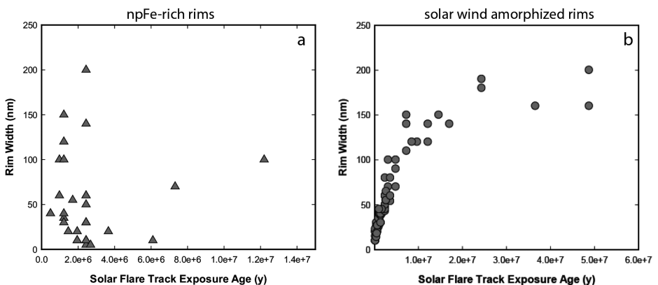
Figure 20. a ) Thickness of npFe-rich rims of anorthite grains from several lunar soils with a range of maturity (67701, 10084, and 62231) vs. the exposure age derived from solar flare tracks for each grain. Rim thickness shows no correlation with exposure age. b ) Solar wind amorphized rims on lunar anorthite grains shows an increase in rim thickness with exposure age until saturation is achieved. After Keller and Zhang (2015).
